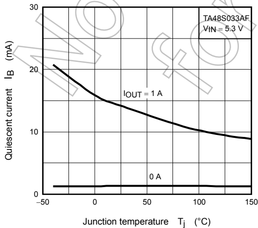
I_B - T_j
